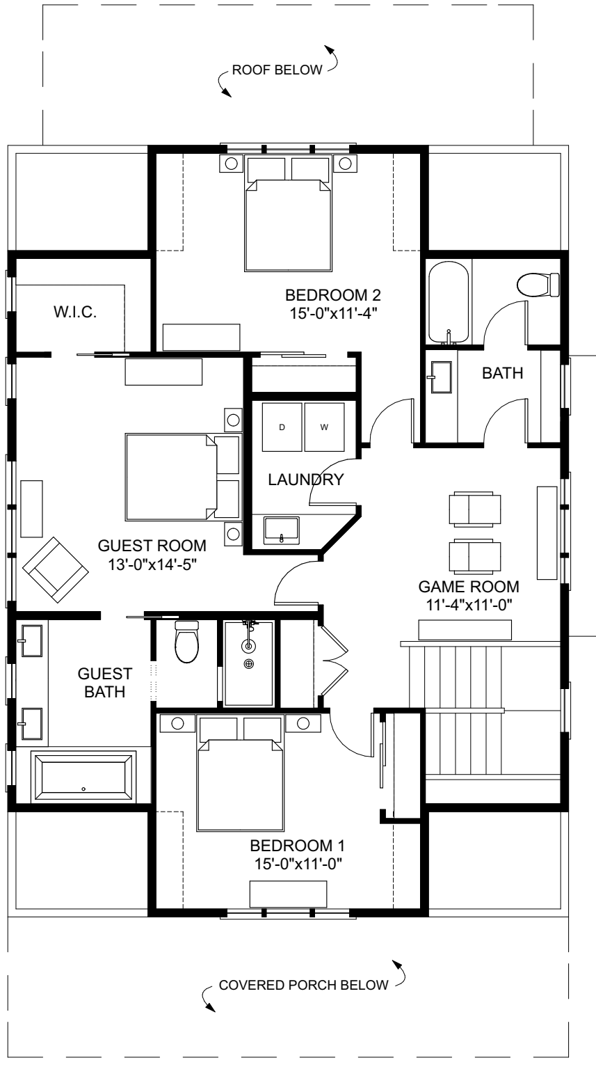
SECOND FLOOR
